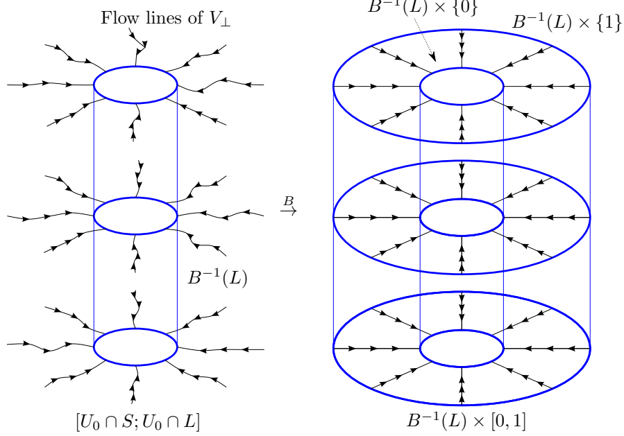
FIGURE 3. The map \psi
