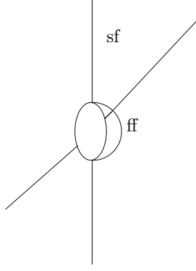
FIGURE 1. The total symbol space S , in the case n = 2 and \mathcal{L} = 0 , with base variables omitted. The front face of the blowup is labeled ff . The side face, labeled sf , is the space S_0 on which principal symbols are defined, and is canonically diffeomorphic to [T^*X; o] . The boundary sphere of this side face is diffeomorphic to SN(o) .
